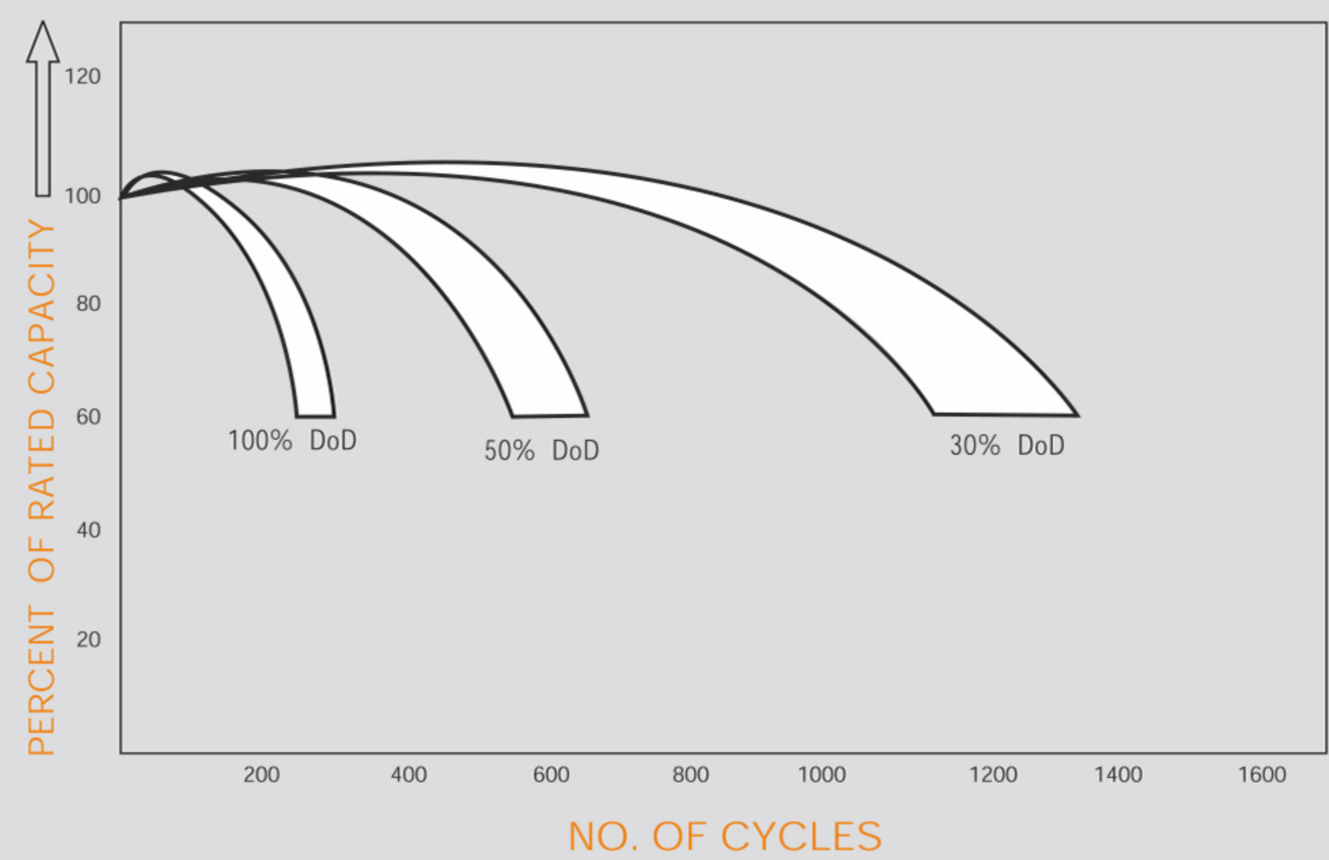
CYCLIC LIFE EXPECTANCY OF AMARON QUANTA™ BATTERIES
